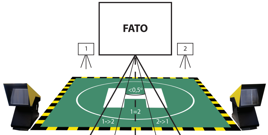
Visual guidance system MS-WSN
